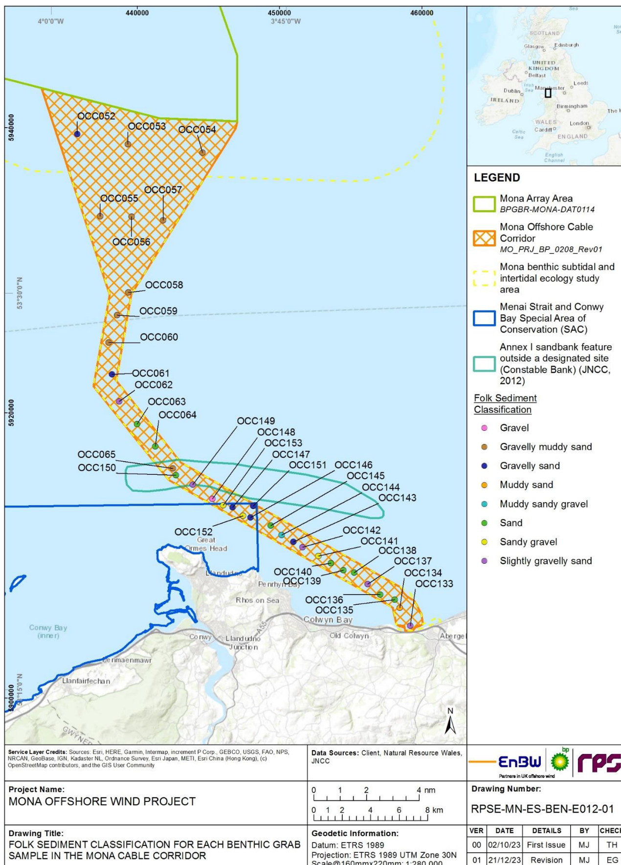
Figure 1.2: Folk sediment classification for each benthic grab sample in the Mona Offshore Cable Corridor.
